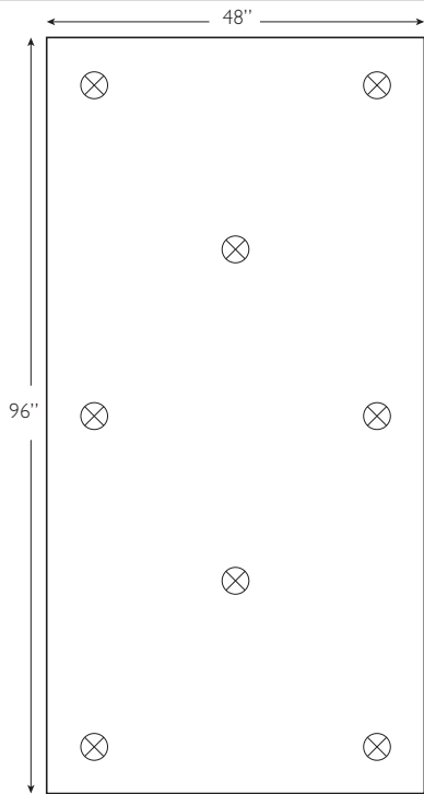
Fasteners should be a minimum of 3" from edge.
